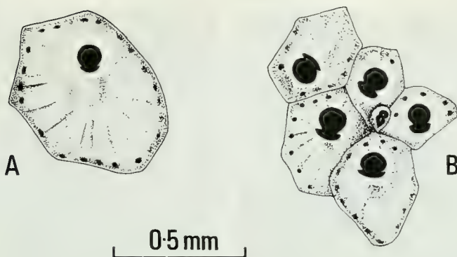
Fig. 4 Hippoporidra edax (Busk). Coralline Crag, Suffolk. A, cortical zooid drawn from the lectotype B1620; B, irregularly-shaped, frontally-budded autozooids and an adventitious avicularium drawn from specimen 23459b.
