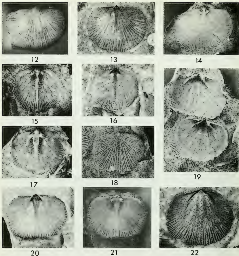
Figs 12–22 Tafilaltia valpyana (Davidson, 1869) from pebbles of late Llandeilo age, Budleigh Salterton Pebble Bed, Devon. Fig. 12, B 21533, latex cast of external mould of a pedicel valve, lectotype (sel. Cocks 1978 : 74), originally figured by Davidson (1869 : pl. 32, fig. 29), \times 2.0 ; W. Vicary Coll. Fig. 13, B 21524, internal mould of a brachial valve, Davidson (1869 : pl. 32, figs 32, 32a), \times 1.8 ; W. Vicary Coll. Fig. 14, B 21509, latex cast of the internal mould of a brachial valve, \times 2.0 . Figs 15, 16, B 21616, latex cast and internal mould of a brachial valve, lectotype of budleighensis (sel. Cocks 1978 : 65), originally figured by Davidson (1870 : pl. 5, fig. 12 lower right), \times 3.0 . Fig. 17, latex cast of the interior of another brachial valve on the same slab as Figs 15 and 16, \times 2.0 . Fig. 18, BB 95940, latex cast of the external mould of a brachial valve, \times 3.0 ; W. Vicary Coll. Fig. 19, B 21621, latex cast of two internal moulds of pedicel valves, \times 3.0 ; W. Vicary Coll. Figs 20, 21, BB 95941, internal mould of a brachial valve and latex cast of it, \times 2.4 ; W. Vicary Coll. Fig. 22, BB 95942, internal mould of a pedicel valve \times 3.0 ; W. Vicary Coll.
