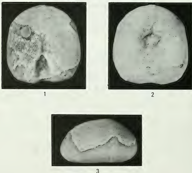
Figs 1-3 Nucleolites clunicularis (Smith). E495, lectotype herein selected, \times 2 . The specimen was coated with ammonium chloride to enhance the detail. 1, apical surface. 2, oral surface. 3, lateral view.
