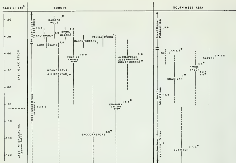
Fig. 2 Ranges of uncertainty in dating Neanderthal and other fossil hominid material of the Upper Pleistocene. The vertical arrangement of sites has no evolutionary significance. 1=indirect ^{14}\text{C} date; 2=uranium series date; 3=direct amino-acid racemization date; 4=amino-acid racemization date (faunal); 5=sedimentological or stratigraphic correlation; 6=faunal correlation. References used in the compilation of this table and not quoted elsewhere are Bräuer (1980), A. J. Jelinek (in press), J. Jelínek (1976), Smith (1976a).
