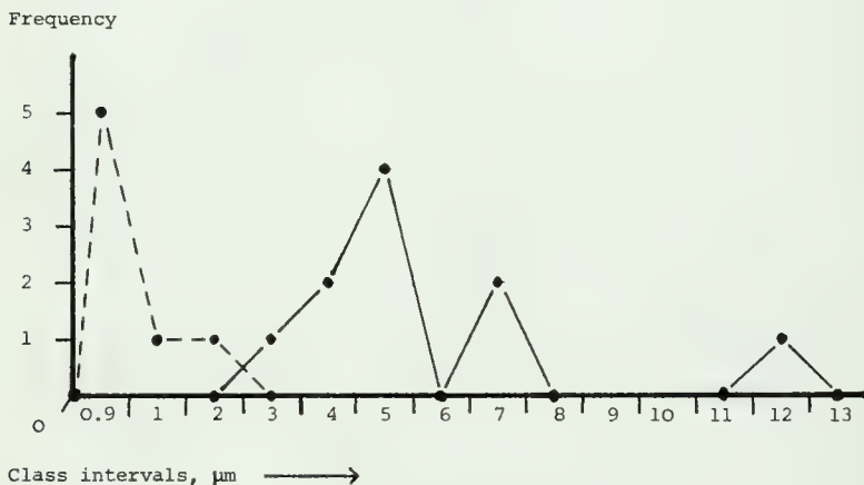
Fig. 8 Internal diameters (a) and tube thicknesses (b) for Girvanella growths in the Stinchar Limestone at Aldons Quarry. Plain lines, maximum range for single growth. Pecked lines, minimum range for single growth.
