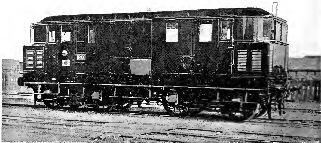
Fig. 281. "BAGGAGE CAR" TYPE OF PARIS-ORLEANS ELECTRIC LOCOMOTIVE.
