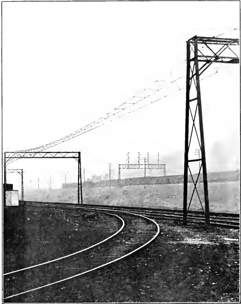
Fig. 224. PHOTOGRAPH SHOWING DOUBLE CABLE SUSPENSION SUPPORTED FROM GANTRIES CONSTRUCTED BY THE WESTINGHOUSE COMPANY.
