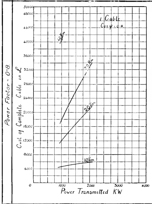
Figs. 125, 126, 127, and 128. CURVES SHOWING MINIMUM COSTS OF CABLES FOR TRANSMITTING 1,000 TO 8,000 K.W. TO A DISTANCE OF 10 TO 40 KILOMETRES. See Fig. 124.
