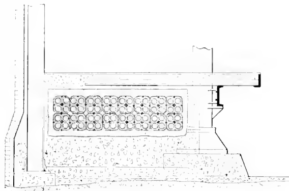
DUCTS UNDER PASSENGER STATION PLATFORM 64 DUCTS Fig. 136. NEW YORK SUBWAY: ARRANGEMENT OF CABLE DUCTS UNDER PASSENGER STATION.
