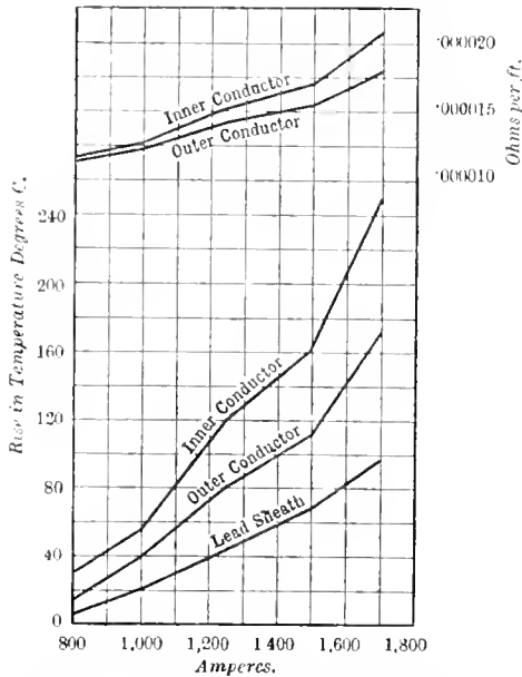
Fig. 131. FERGUSON'S TESTS OF TEMPERATURE DISTRIBUTION IN CABLES.
