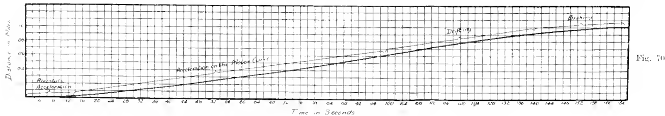
FIGS. 67-70. ACCELERATION-CURRENT-SPEED-DISTANCE-TIME CURVES FOR FOUR G. E. 66 A MOTORS IN PARALLEL.
