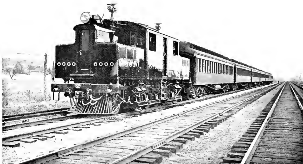
Fig. 262. NEW YORK CENTRAL LOCOMOTIVE HAULING A SIX-CAR TRAIN DURING ONE OF THE TESTS OF NOVEMBER, 1904.
