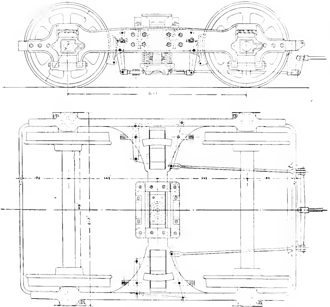
Fig. 111. CENTRAL LONDON RAILWAY: CAST STEEL TRAILER BOGIES. GENERAL ARRANGEMENT OF MCGUIRE TRUCK.
