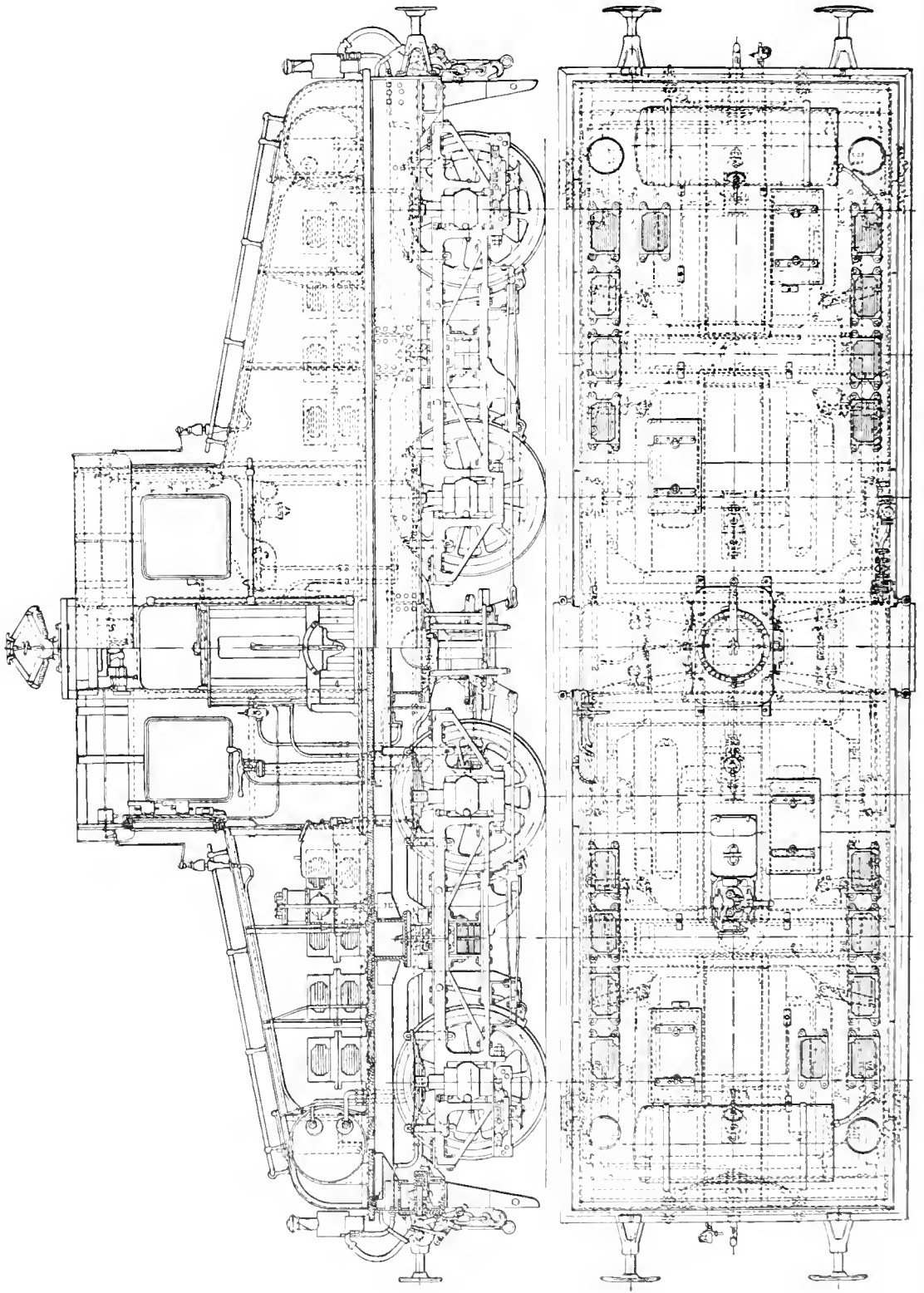
FIG. 277. 49 METRIC-TON PARIS-ORLEANS GEARED ELECTRIC LOCOMOTIVE.
