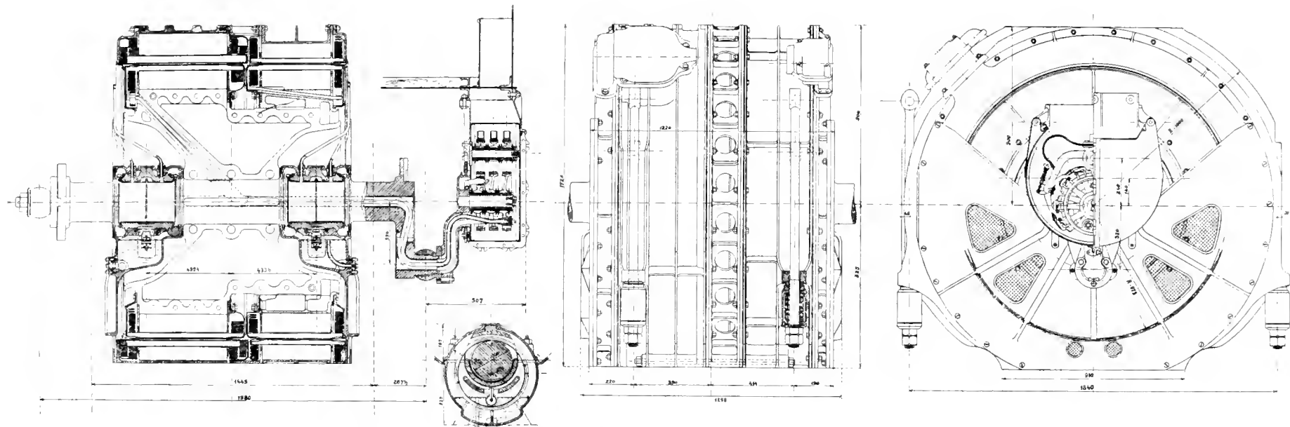
Fig. 208. OUTLINE DRAWINGS OF ONE OF THE CASCADE MOTOR SETS OF THE "1904" TYPE VALIELLINA THREE-PHASE ELECTRIC LOCOMOTIVE.
