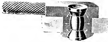
Fig. 237. GENERAL ELECTRIC Co. (U.S.A.) RAIL BOND: SECTION THROUGH BOND, SHOWING EFFECT OF COMPRESSION.
