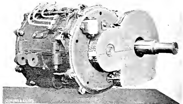
Fig. 330. SIEMENS AND HALSKE 10,000-VOLT THREE-PHASE MOTOR.
