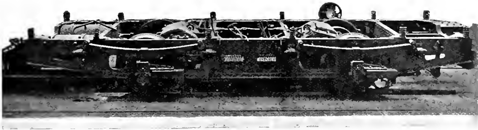
Fig. 398. TRUCK OF PARIS-METROPOLITAN MOTOR CAR WITH RIGID WHEEL BASE.
