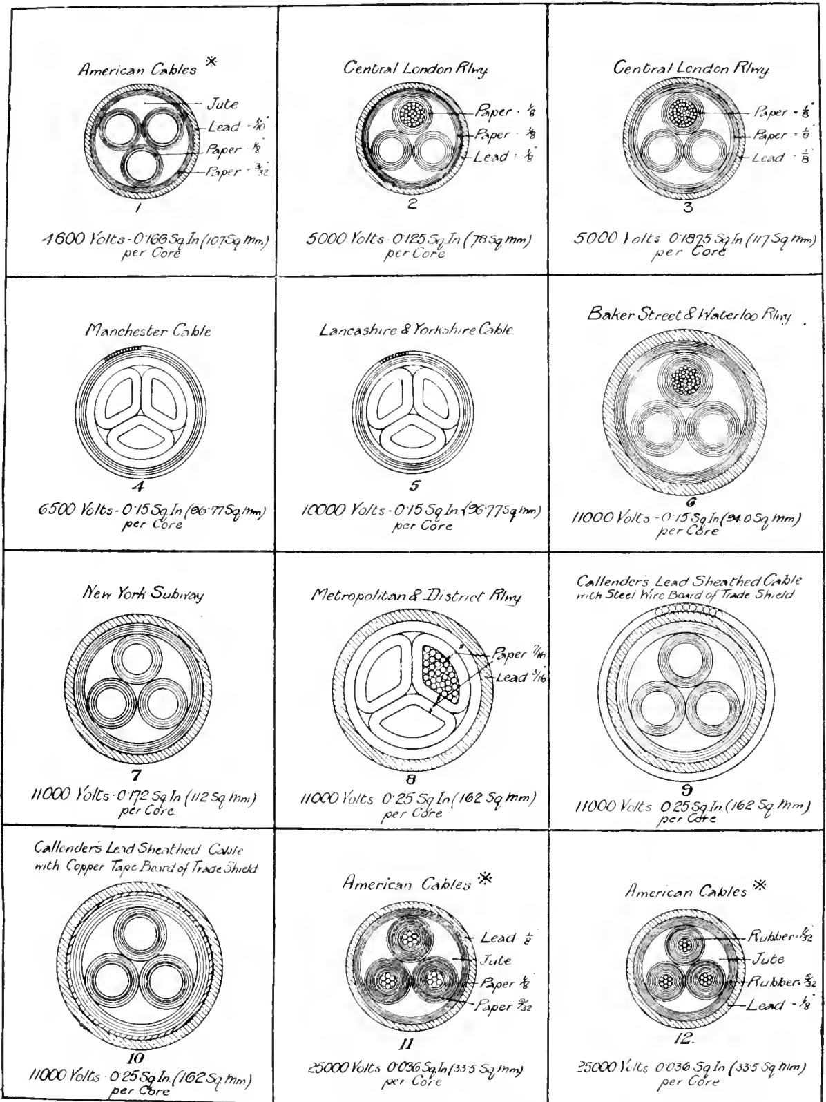
Fig. 143. SECTIONS OF VARIOUS HIGH TENSION CABLES.
