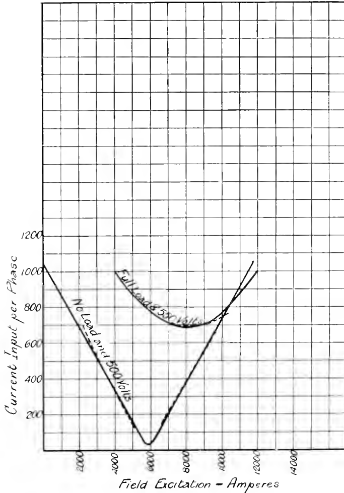
Fig. 168. 100-K.W. ROTARY CONVERTER CHARACTERISTIC PHASE CURVES.
