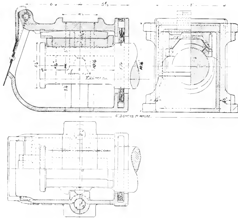
Fig. 423. MASTER CAR-BUILDERS' STANDARD AXLE-BOX FOR A 4\frac{1}{2} IN. JOURNAL.
