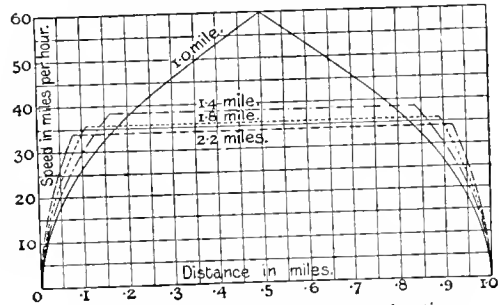
C—Speed-Distance Curves for same accelerations
