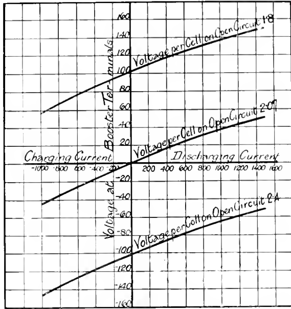
Fig. 169. BOOSTER VOLT-AMPERE CHARACTERISTIC CURVES.
