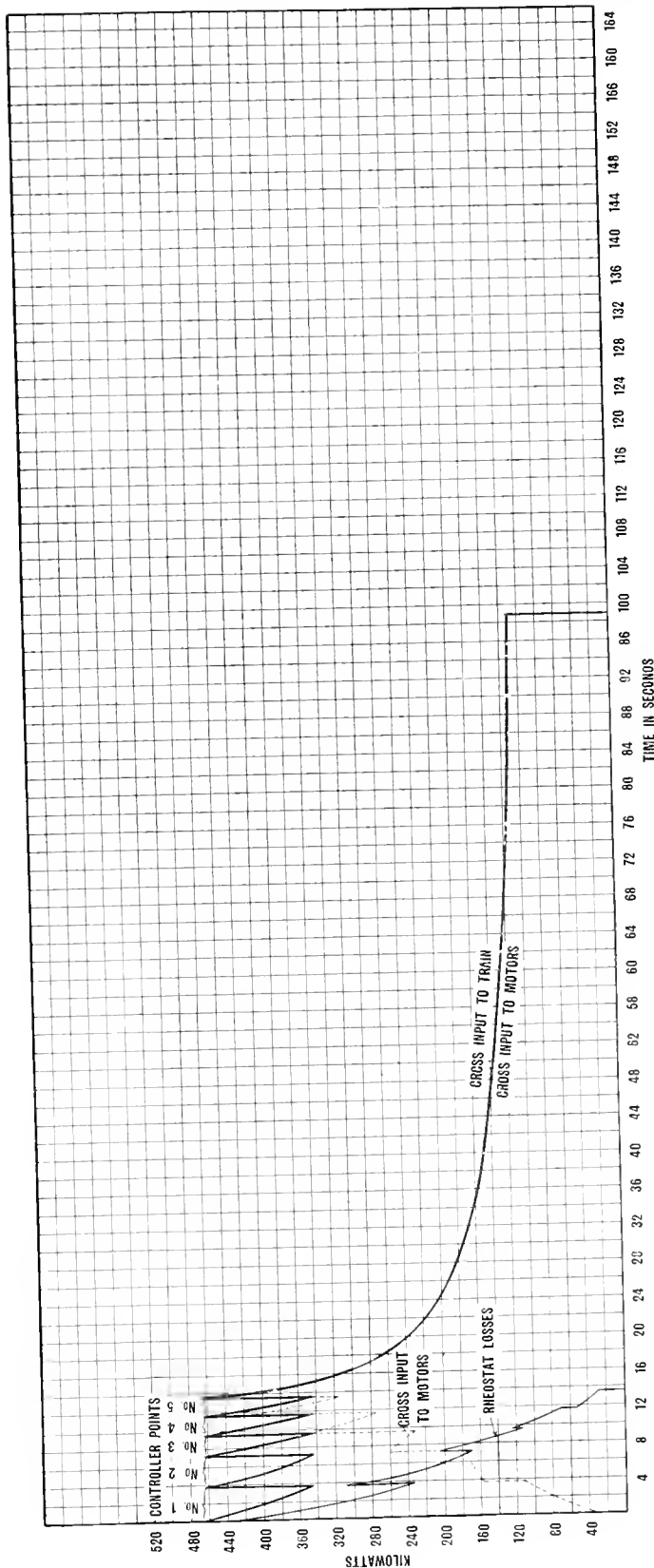
Fig. 71. CURVES ALLOCATING THE DISTRIBUTION OF THE ENERGY WITH FOUR G6 A MOTORS IN PARALLEL.
