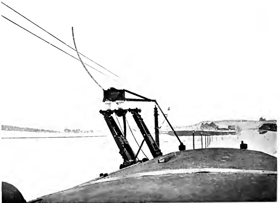
Fig. 318. OERLIKON TROLLEY.
