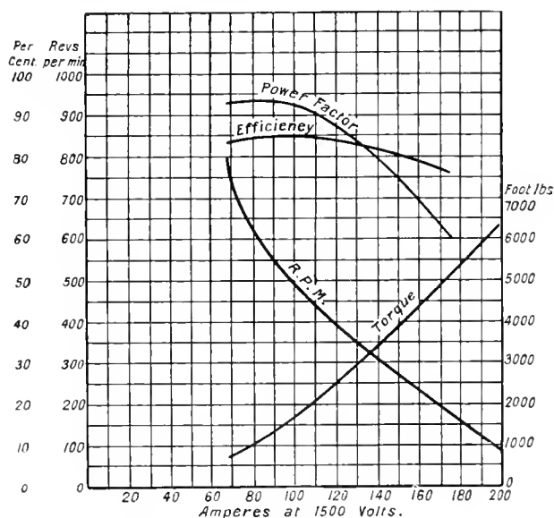
Fig. 392. CALCULATED CURVE OF 175 H.-P. REPUulsion MOTOR AT 1,500 VOLTS.
