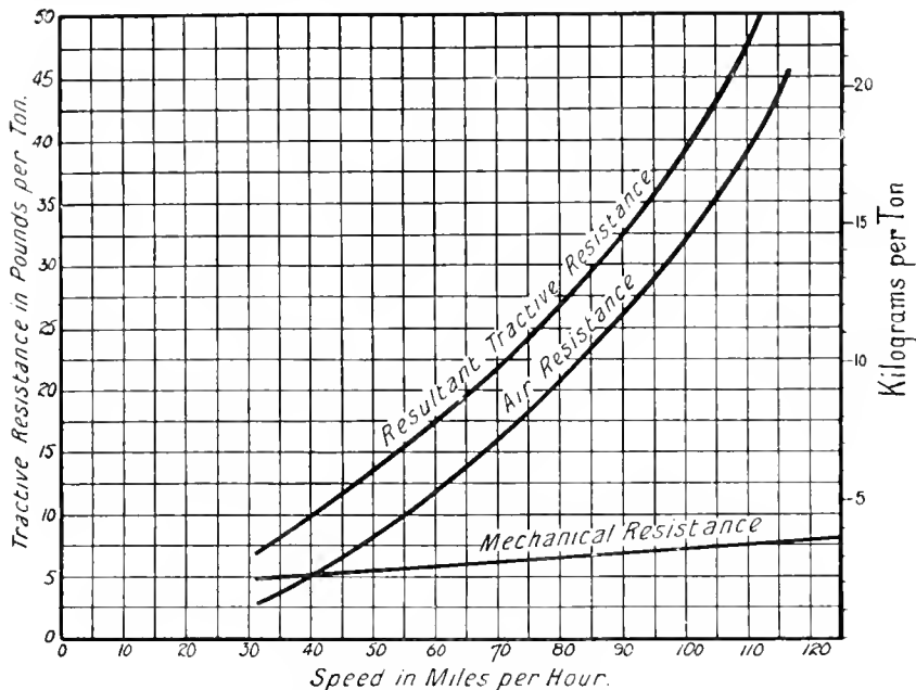
Fig. 8. CURVES OF COMPONENT AND RESULTANT TRACTIVE RESISTANCE FOR 83-TON 75-FOOT CAR, DEDUCED FROM BERLIN-ZOSSFEN TESTS.
