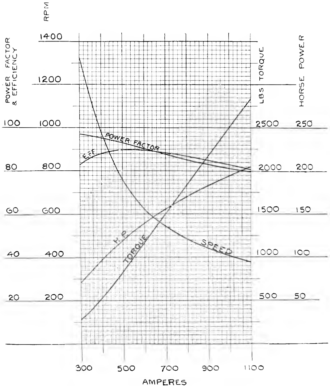
Fig. 371. CHARACTERISTIC CURVES OF BRITISH WESTINGHOUSE ELECTRIC AND MANUFACTURING Co's STANDARD SINGLE-PHASE RAILWAY MOTOR.
