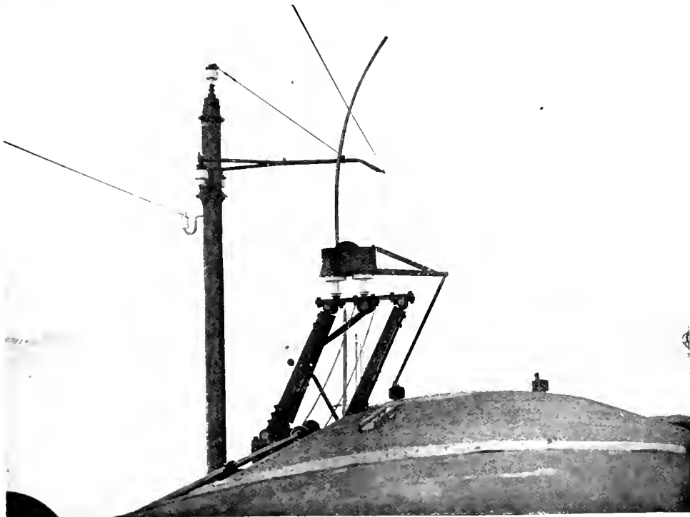
Fig. 320. OERLIKON TROLLEY.
