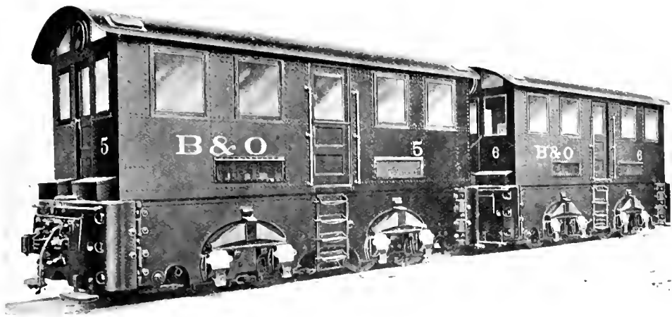
Fig. 270. BALTIMORE AND OHIO TWO-UNIT 1903 LOCOMOTIVE, WITH GEARED FOUR-POLE MOTORS. WEIGHT OF TWO-UNIT COMBINATION, 146 TONS.
