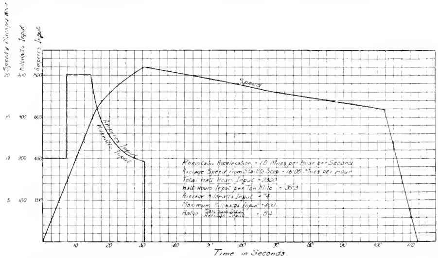
Fig. 92. CHARACTERISTIC CURVES FOR A \frac{1}{2} -MILE RUN AT AN AVERAGE SPEED OF 16.1 MILES PER HOUR. 120-TON TRAIN. LEVEL TRACK. COASTING FOR 72 SECONDS.
