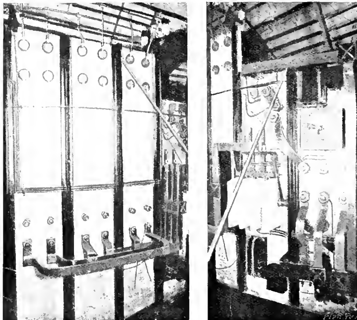
Converter Panel.
