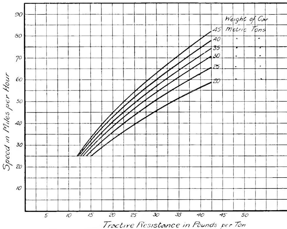
Fig. 106. CURVES OF TRACTIVE RESISTANCE FOR SINGLE CARS OF VARIOUS WEIGHTS ACCORDING TO WYNNE. (Blood's Formula.)
