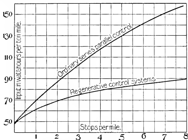
Fig. 11. CURVES FOR TRAMCAR OPERATED ON ORDINARY SERIES PARALLEL AND ON REGENERATIVE CONTROL SYSTEMS.
