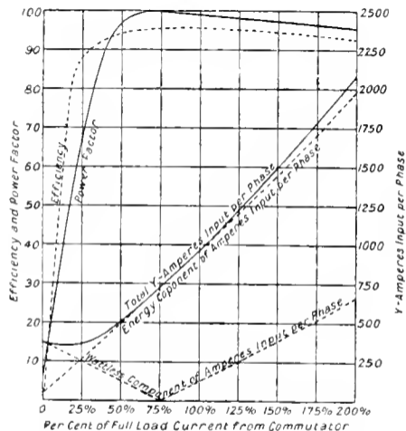
Rotary Converter with 30 per cent. Compounding.
