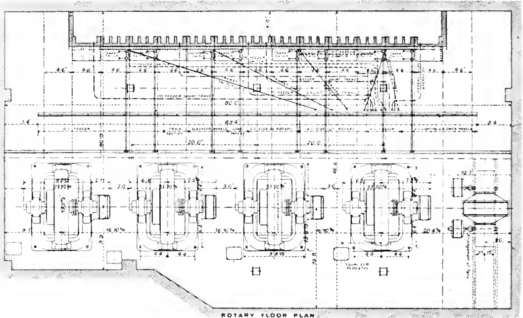
Fig. 196. DISTRICT RAILWAY: PLAN OF CHARING CROSS SUB-STATION.
