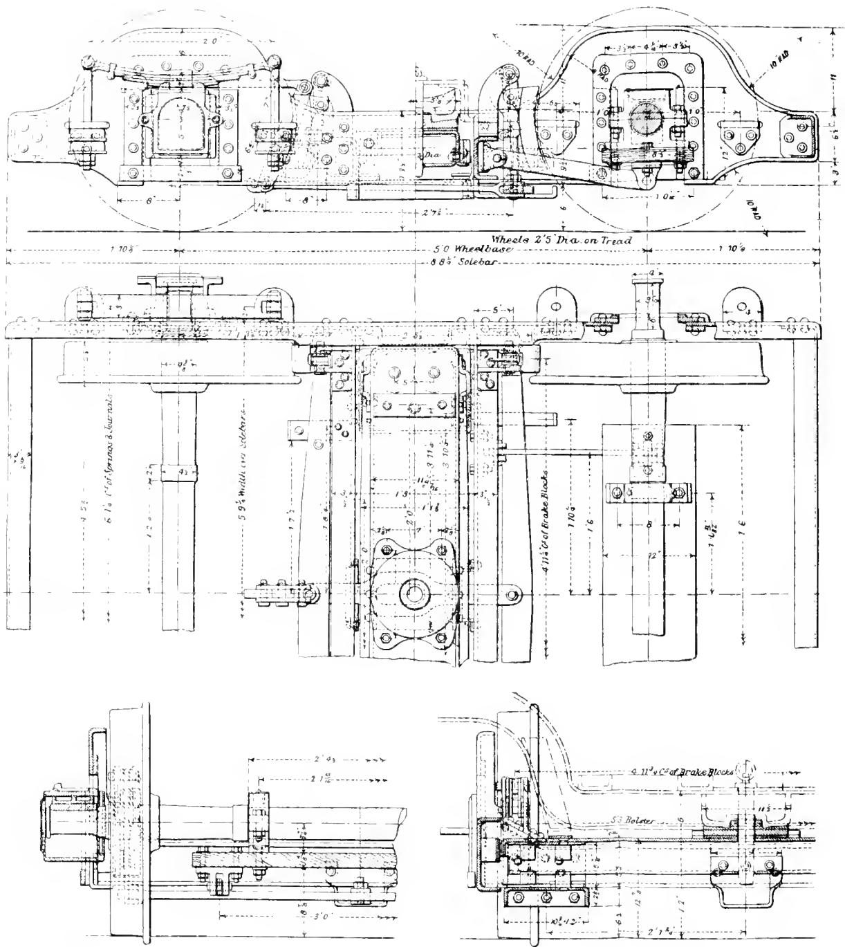
Fig. 415. BOGIE TRUCK UNDER TRAILER END OF CENTRAL LONDON RAILWAY CARRIAGE.
