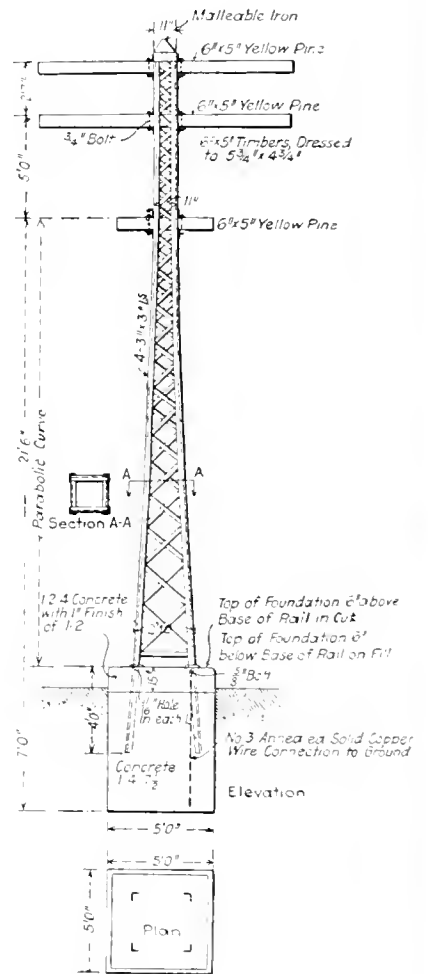
FIG. 145A. NEW YORK CENTRAL RAILWAY: PLAN, ELEVATION, AND SECTIONS OF POLE FOR TRANSMISSION LINES.
