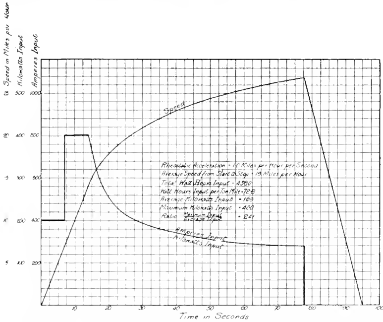
Fig. 90. CHARACTERISTIC CURVES FOR A \frac{1}{2} -MILE RUN AT AN AVERAGE SPEED OF 19 MILES PER HOUR, 120-TON TRAIN, LEVEL TRACK, NO COASTING.
