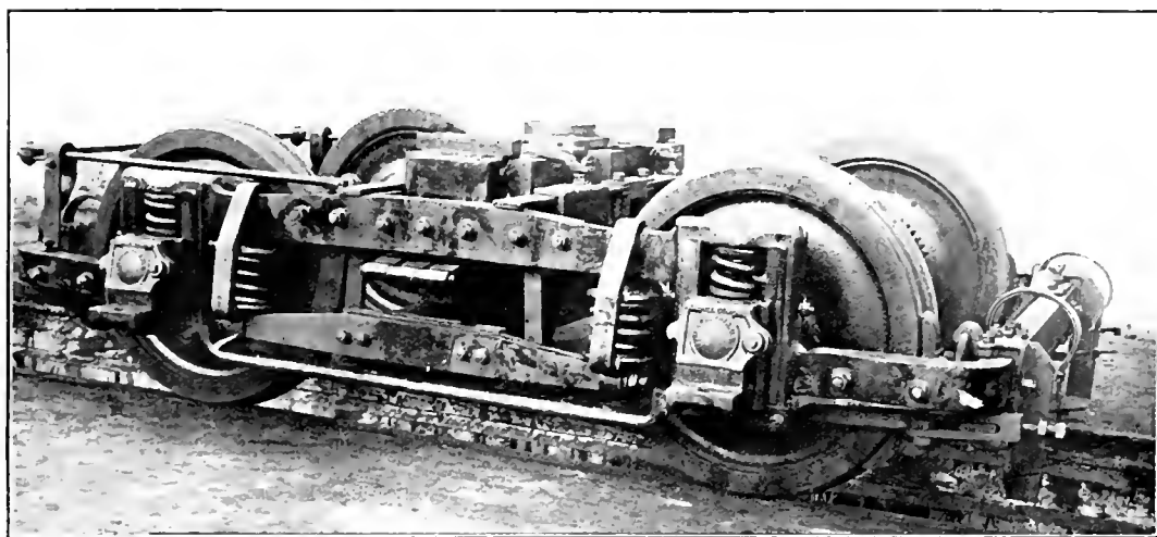
Fig. 413. BRILL TRUCK.
